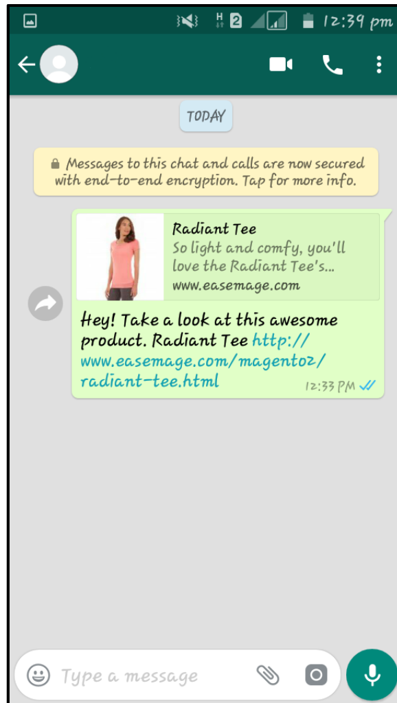
Figure 3 – WhatsApp
